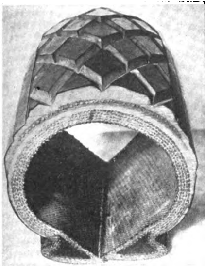
SECTION AJAX NON-SKID TIRE.
